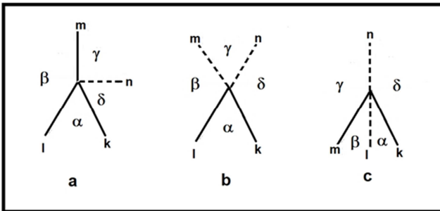
Figure 2. Mapping the Gibbs function topological manifold for a binary system onto the plane ( p, T ) creates a graph-map of three invariant states that are possible in the binary states (a, b, c). The edges of the graph-map, i.e. the lines k, l, m, n that bifurcate in an invariant state, are given by Equations (5) and are composed of segments \alpha, \beta, \gamma, \delta which determine the equilibrium of each phase. Component A (specifically, the chemical potential of Component A) is marked in the graph with a continuous line, and Component B is marked with a dashed line. Phase compositions in figures a, b, c give Eq.(6).
